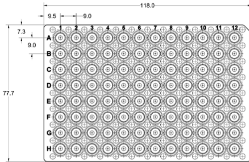
Dimensions are millimeters. Do not scale
