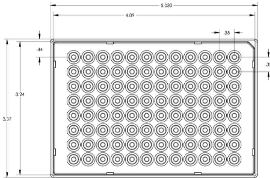
Dimensions are inches. Do not scale
