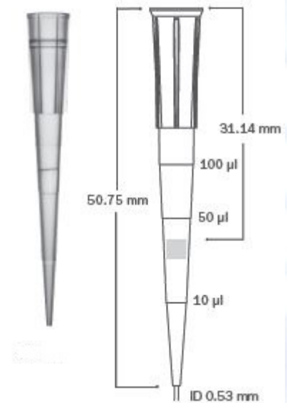
Filter Tip
