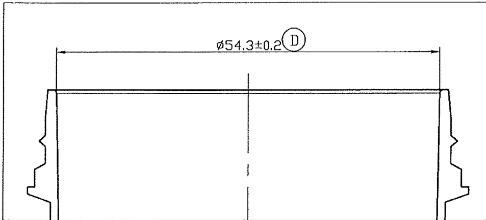
NECK DETAIL SCALE 2
