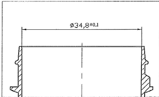
NECK DETAIL SCALE 2
