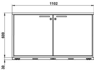
Vue de face UB90.060.110.050.2T
