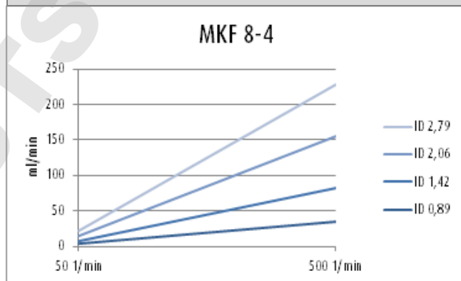
Flow rates in combination with series 80
