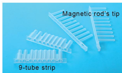
Auto-Pure20A consumables
