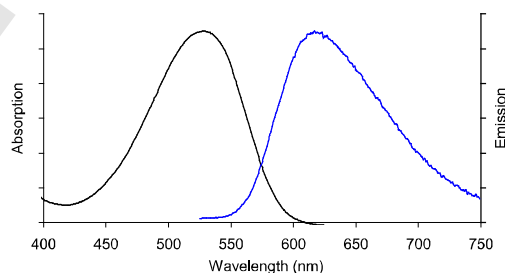
Absorption and emission of EthD-III bound to DNA
