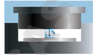
Sample Window System with Nano Hydrophobic Coating
