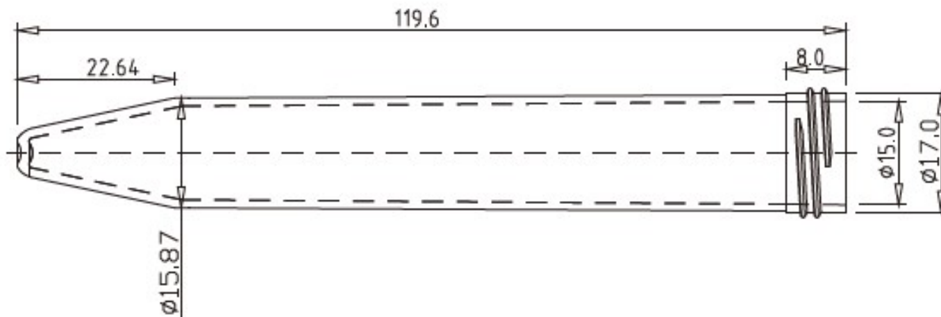
Plug seal cap
