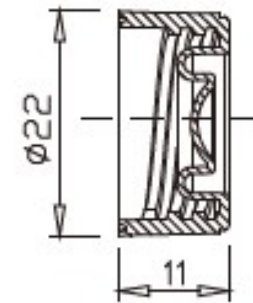
Plug seal cap
