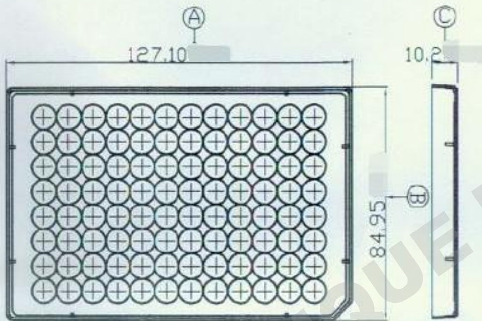
96-F Well Lid
