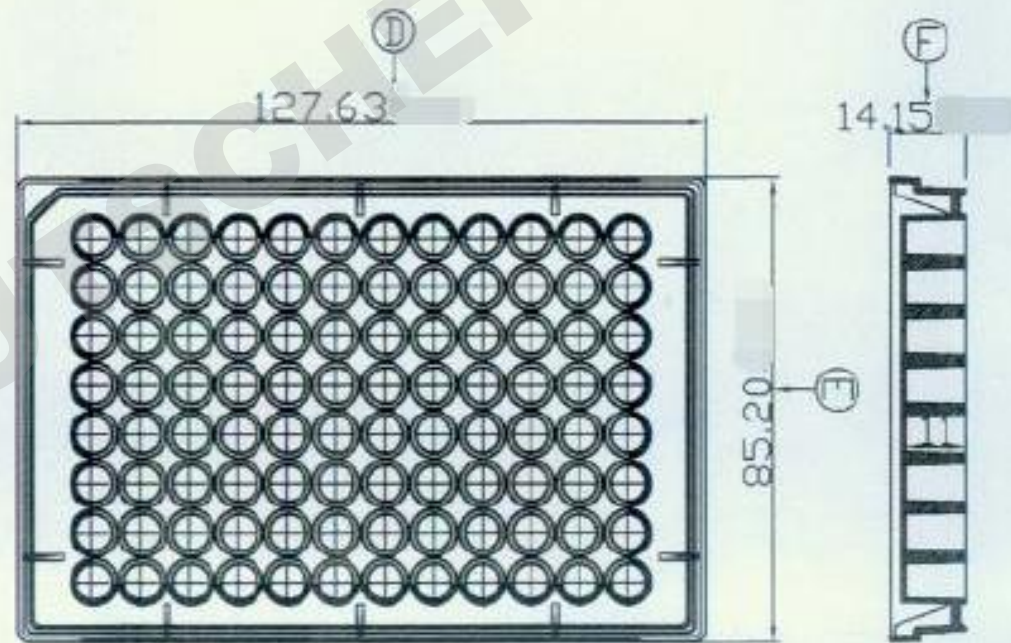
96-F Well Plate
