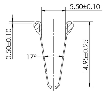
VIAL FORM
