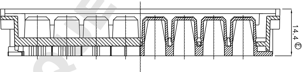
Section CC
