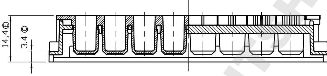
Section CC
