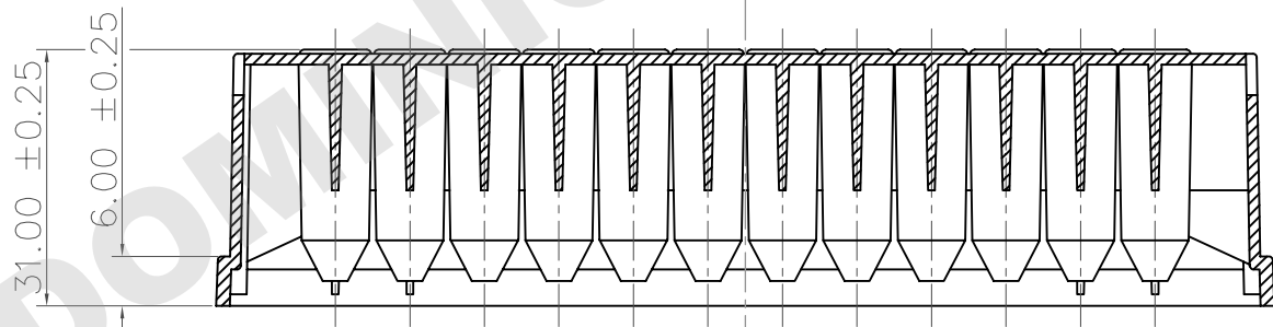
SECTION X-X
