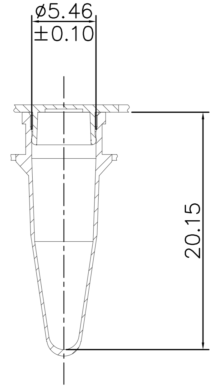
SECTION thro' TUBE & CAP 8pos
