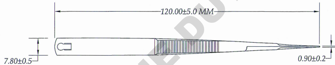
SIDE ELEVATION
